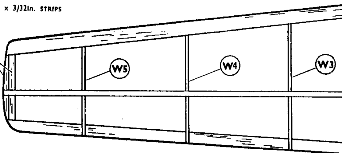
Fig. 3 BULK STRIP ASSEMBLY
