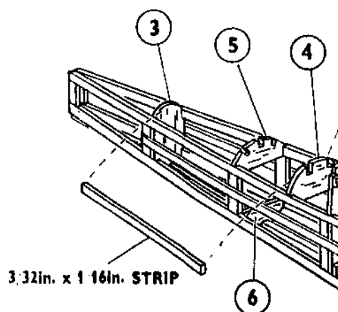
Fig. 3 BULK STRIP ASSEMBLY
