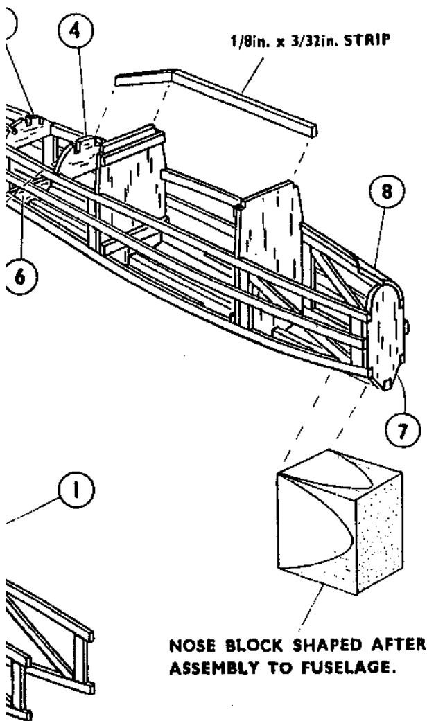
g. 3 BULKHEADS, PARTS 8, STRINGERS AND NOSE BLOCK ASSEMBLED.
